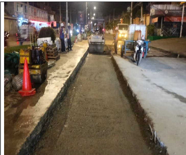
Base course backfilling and compaction
