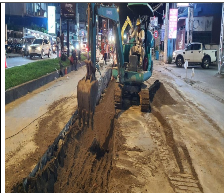
Photo: 07 Sand backfilling and compaction
