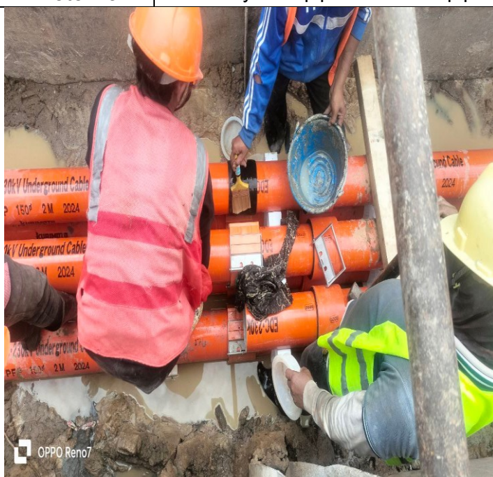
Photo: 22 Assembly PFP pipes and OFC pipe
