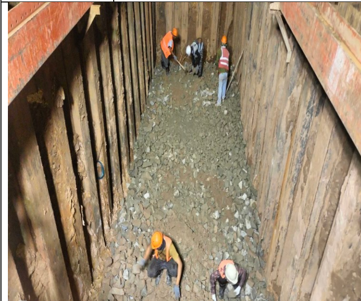
Manhole Installation activity
