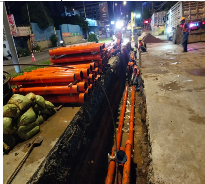
Photo: 03 Assembly PFP pipes and OFC pipe
