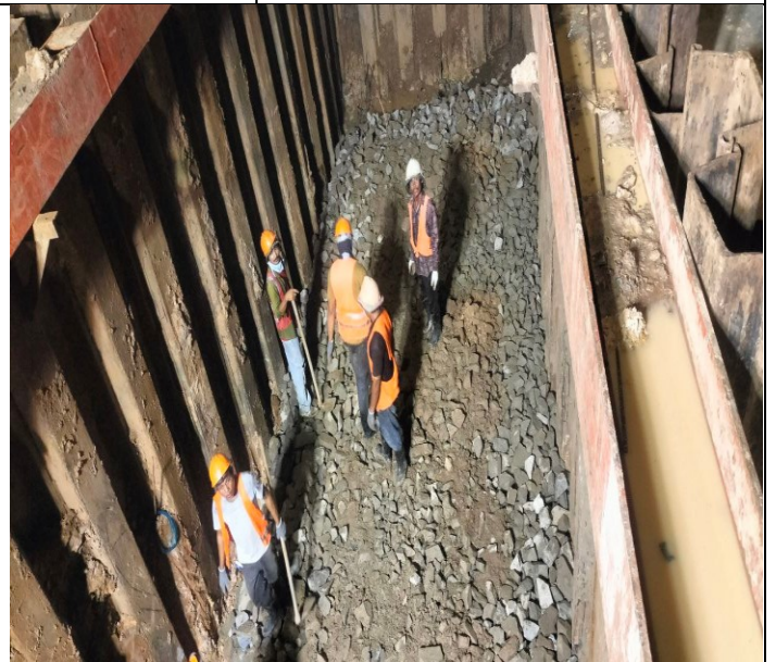
Manhole Installation activity
