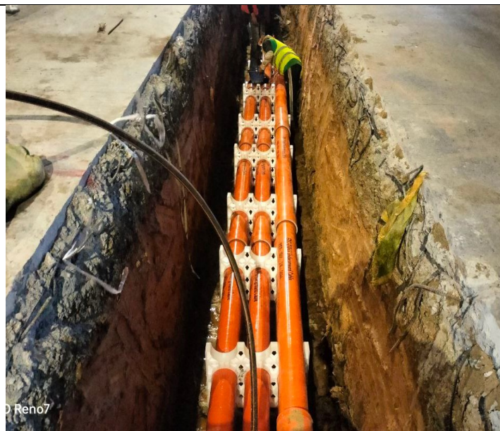
Photo: 08 Assembly PFP pipes and OFC pipe
