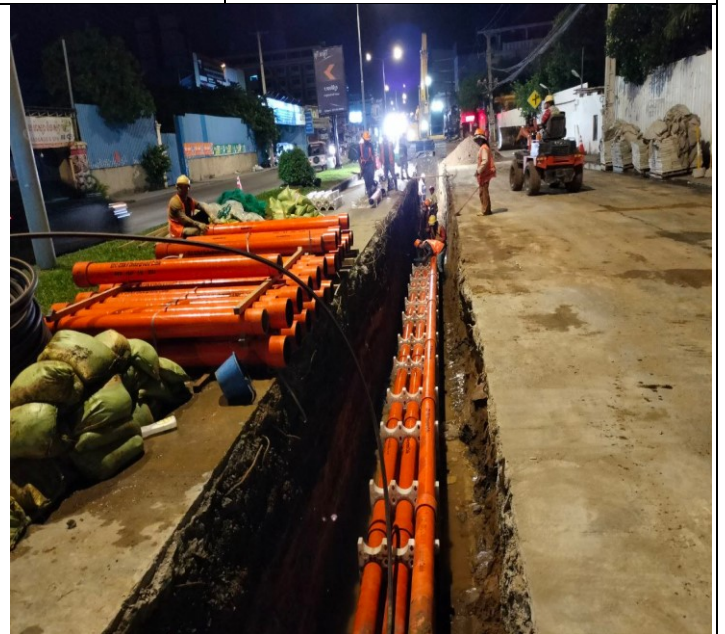
Photo: 04 Assembly PFP pipes and OFC pipe
