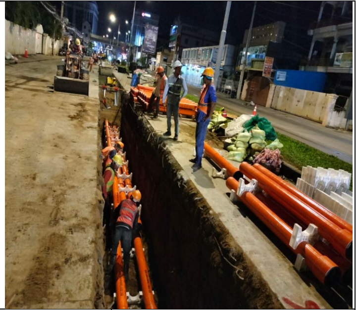
Photo: 02 Assembly PFP pipes and OFC pipe
