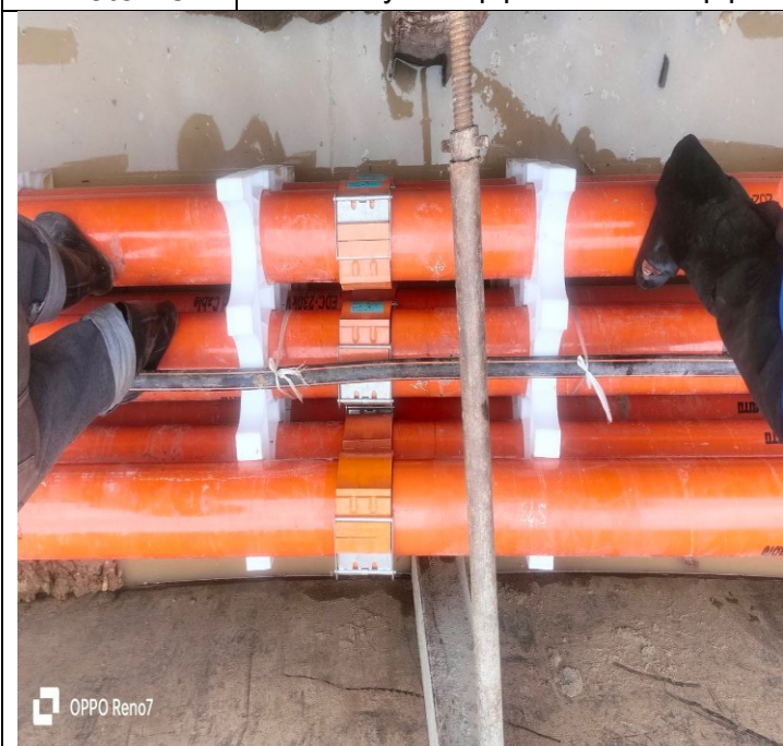
Photo: 21 Assembly PFP pipes and OFC pipe
