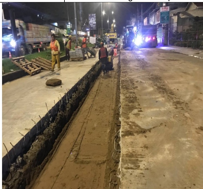
Photo: 12 Sand backfilling and compaction
