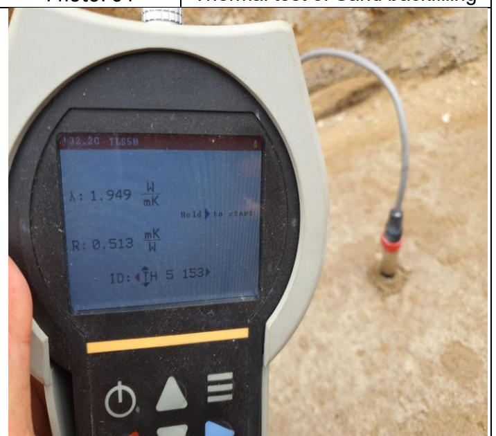
Photo: 06 Thermal test of Sand backfilling
