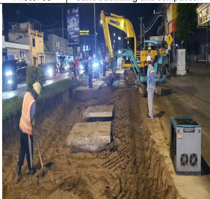
Photo: 10 Sand backfilling and compaction
