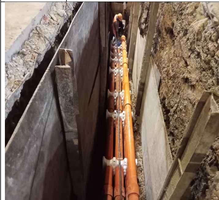
Photo: 11 Assembly PFP pipes and OFC pipe
