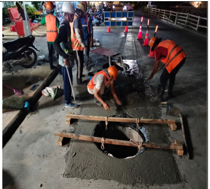
Photo: 08 Manhole Cover Installation activity
