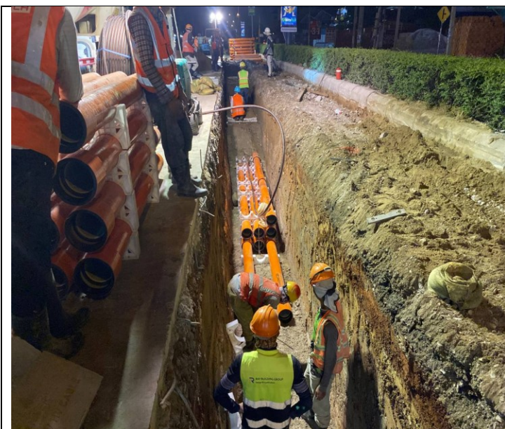
Photo: 07 Assembly PFP pipes and OFC pipe
