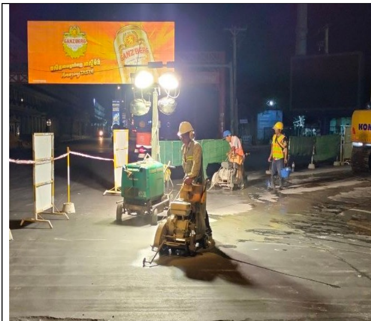
Photo: 03 Saw cutting of concrete road
