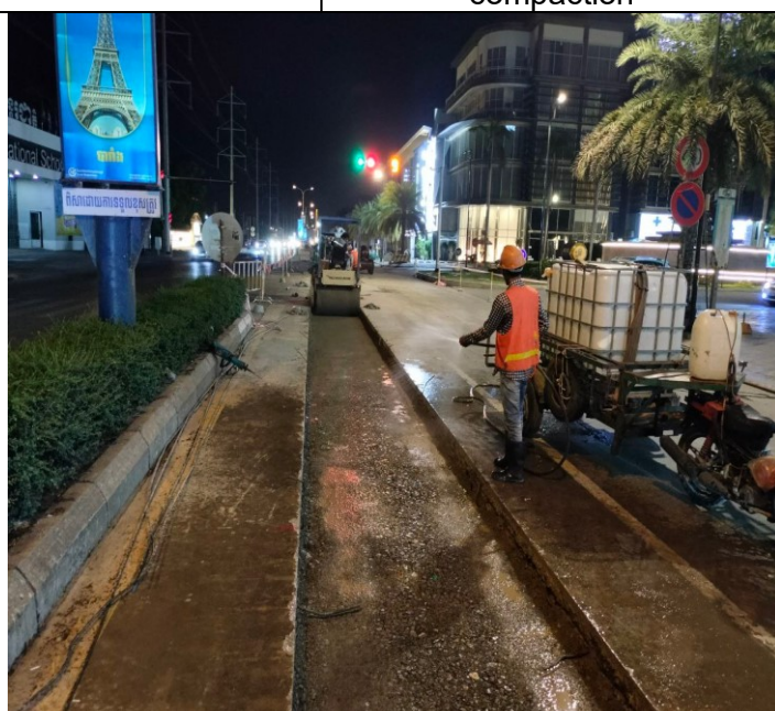
Base course backfilling and compaction
