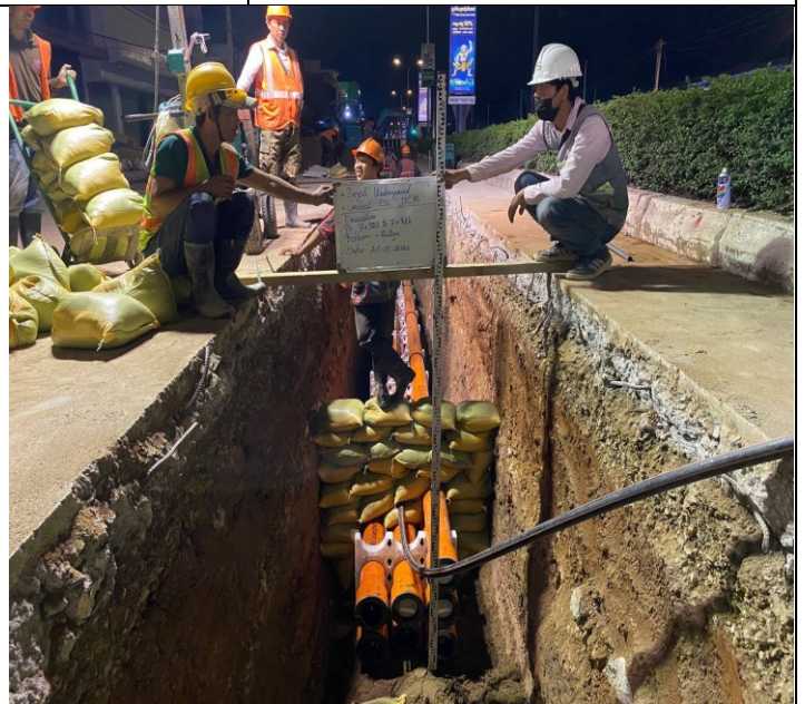
Photo: 18 Assembly PFP pipes and OFC pipe
