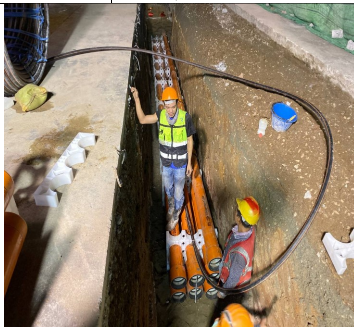
Photo: 12 Assembly PFP pipes and OFC pipe
