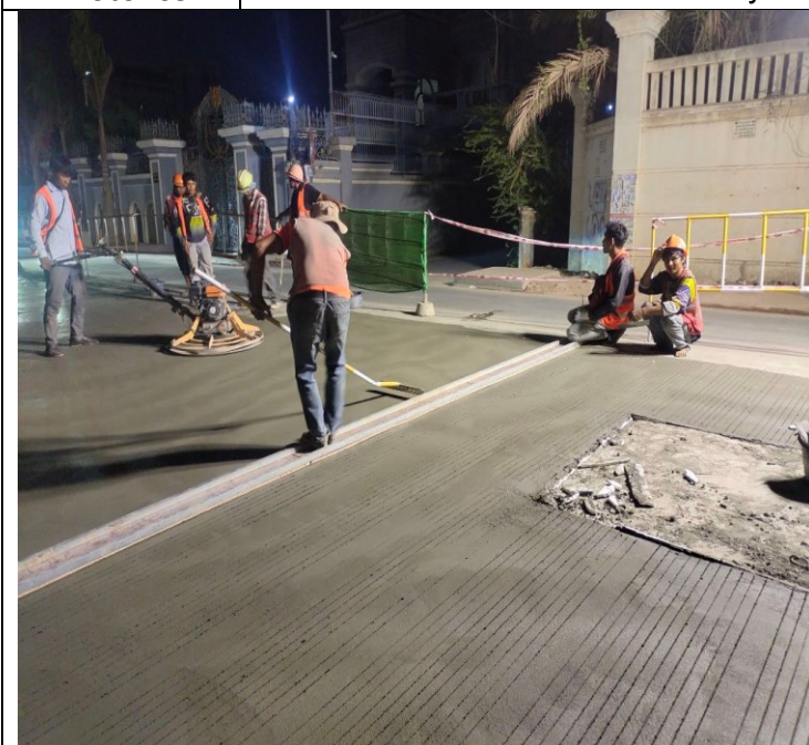
Photo: 11 Manhole of concrete road activity
