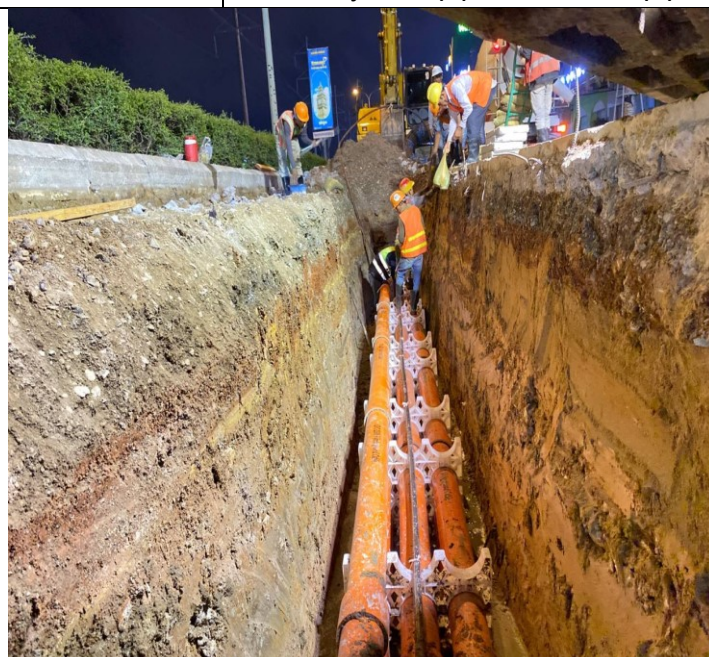
Photo: 10 Assembly PFP pipes and OFC pipe
