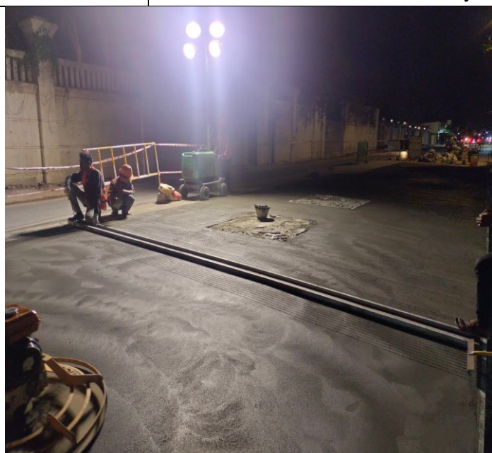
Photo: 10 Manhole of concrete road activity
