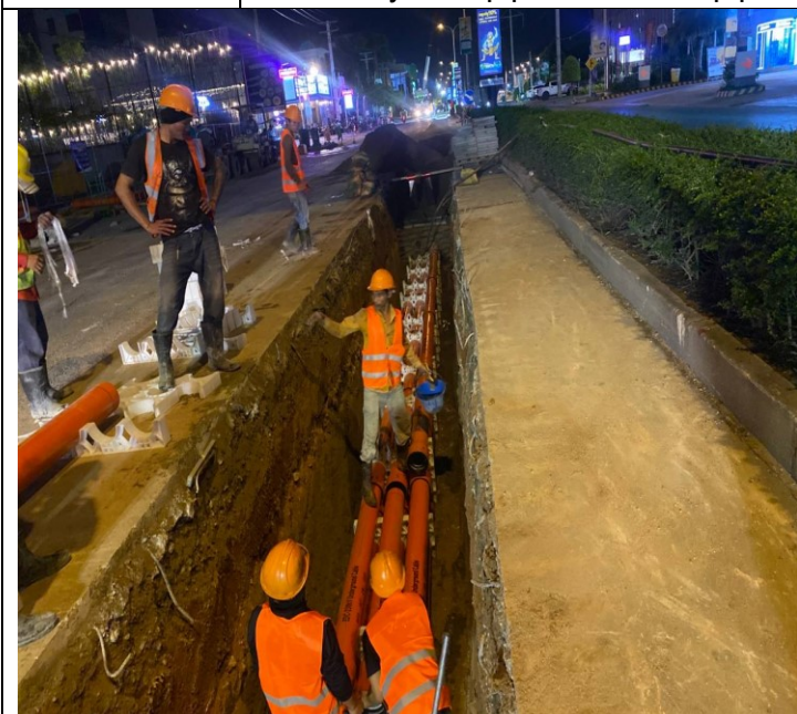
Photo: 29 Assembly PFP pipes and OFC pipe
