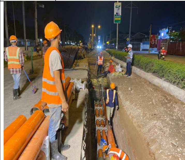
Photo: 05 Assembly PFP pipes and OFC pipe
