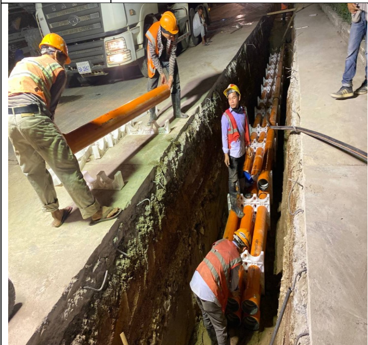
Photo: 23 Assembly PFP pipes and OFC pipe
