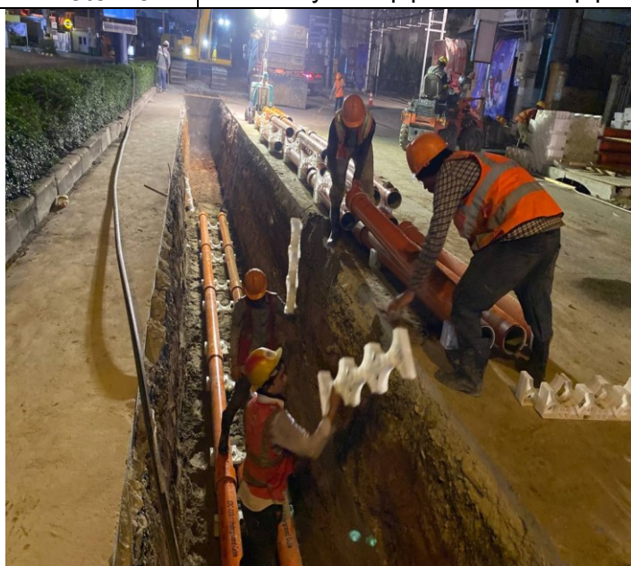
Photo: 22 Assembly PFP pipes and OFC pipe
