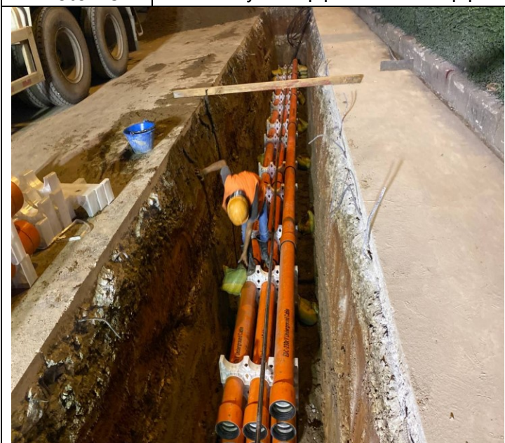
Photo: 21 Assembly PFP pipes and OFC pipe
