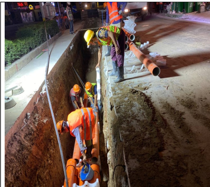
Photo: 25 Assembly PFP pipes and OFC pipe
