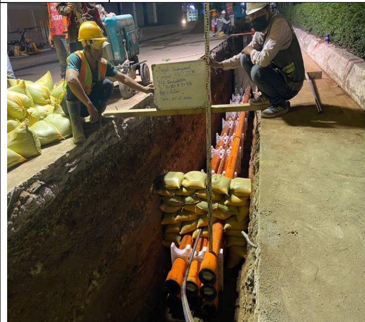
Photo: 17 Assembly PFP pipes and OFC pipe
