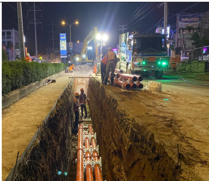
Photo: 20 Assembly PFP pipes and OFC pipe
