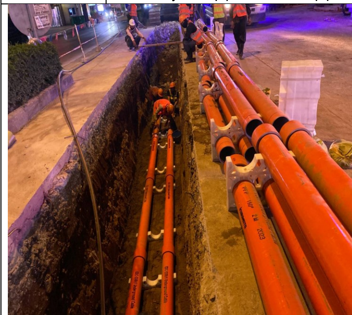
Photo: 27 Assembly PFP pipes and OFC pipe
