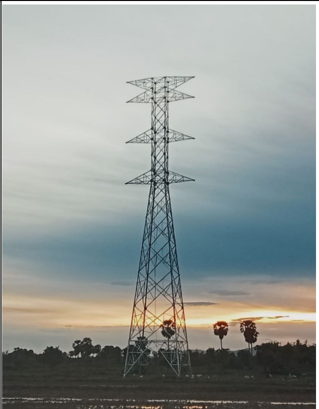
TA106 Tower erection completed .
