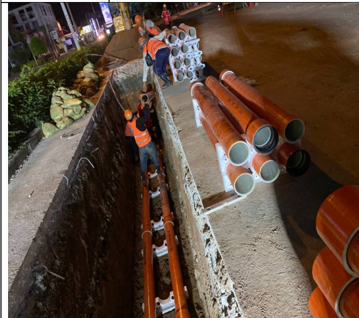
Photo: 15 Assembly PFP pipes and OFC pipe
