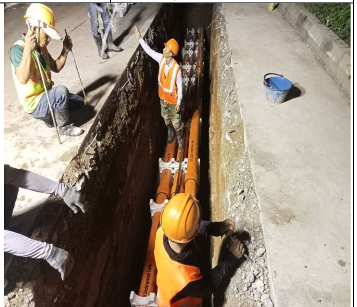
Photo: 06 Assembly PFP pipes and OFC pipe
