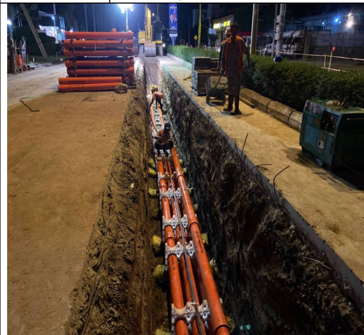
Photo: 29 Assembly PFP pipes and OFC pipe
