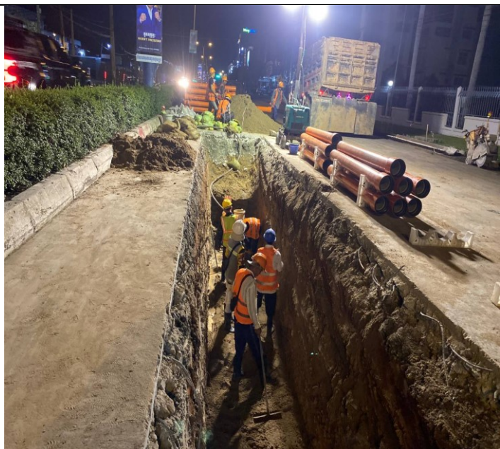
Photo: 26 Assembly PFP pipes and OFC pipe
