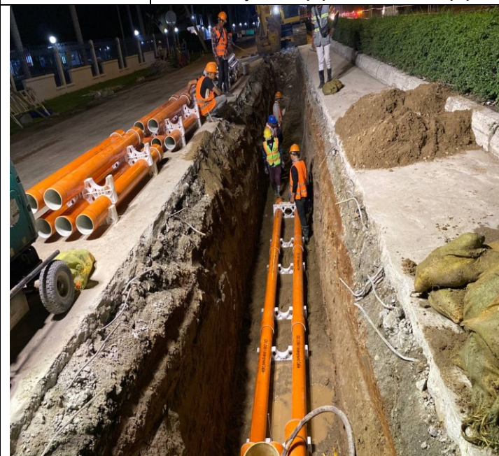
Photo: 27 Assembly PFP pipes and OFC pipe
