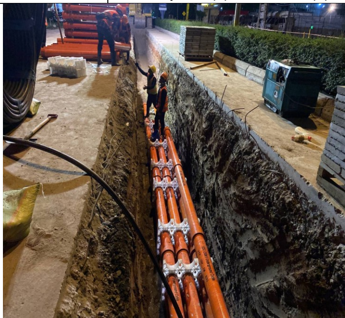
Photo: 28 Assembly PFP pipes and OFC pipe
