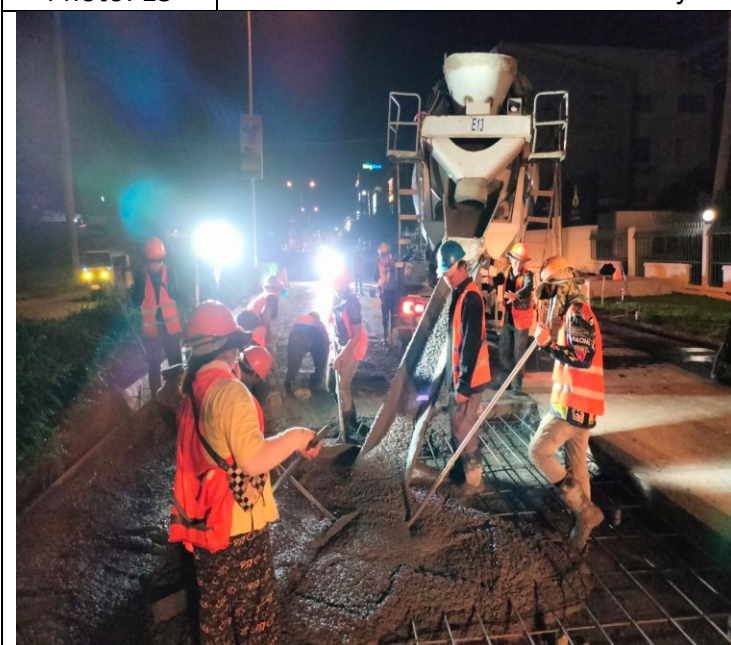
Photo: 15 Manhole of concrete road activity
