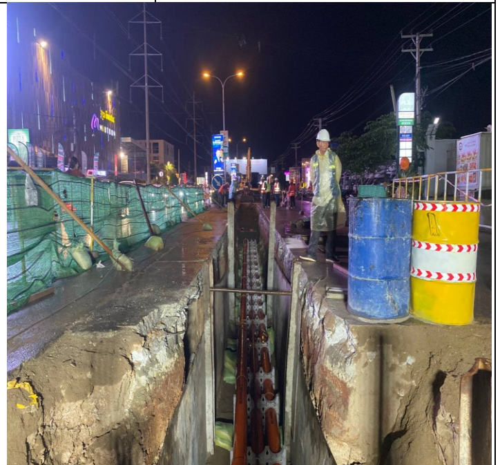
Photo: 24 Assembly PFP pipes and OFC pipe
