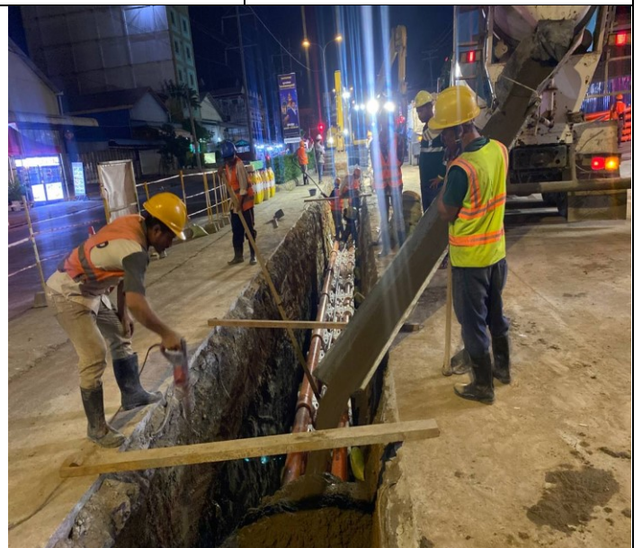
CBS casting (mortar)
