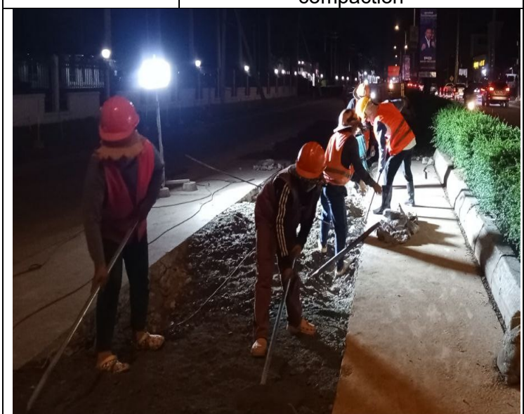
Base course backfilling and compaction
