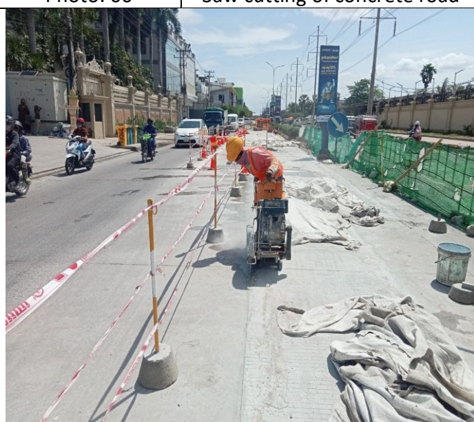
Photo: 08 Saw cutting of concrete road
