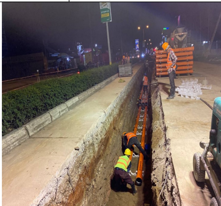
Photo: 30 Assembly PFP pipes and OFC pipe
