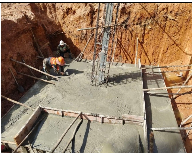
Concrete leveling .
