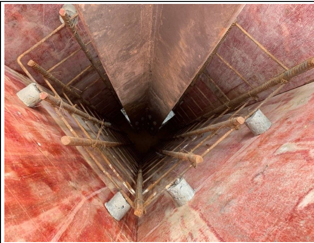
Cover concrete .
