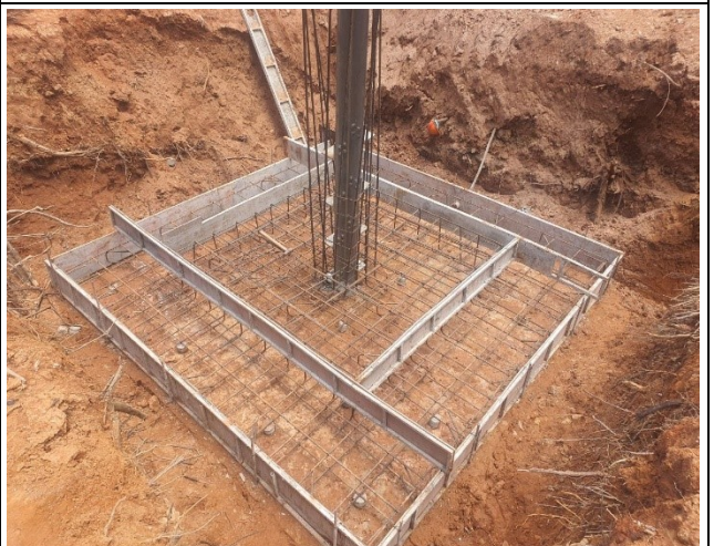
Install rebar and formworks.
