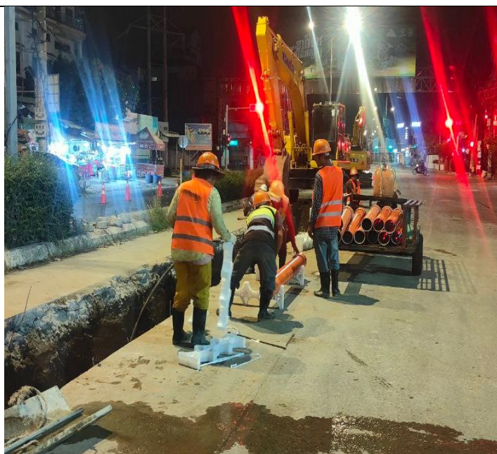
Photo: 14 Assembly PFP pipes and OFC pipe
