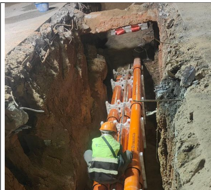
Photo: 13 Assembly PFP pipes and OFC pipe
