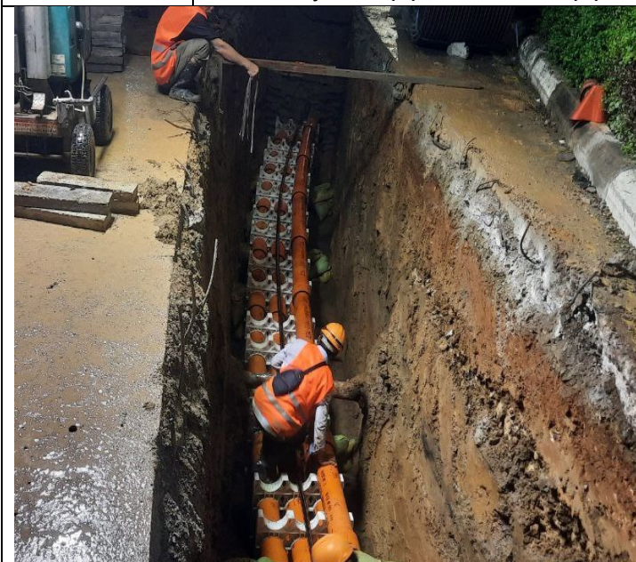
Photo: 23 Assembly PFP pipes and OFC pipe
