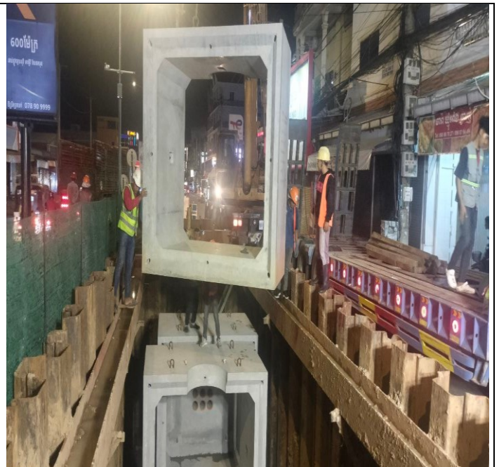
Photo: 20 Manhole Installation activity
