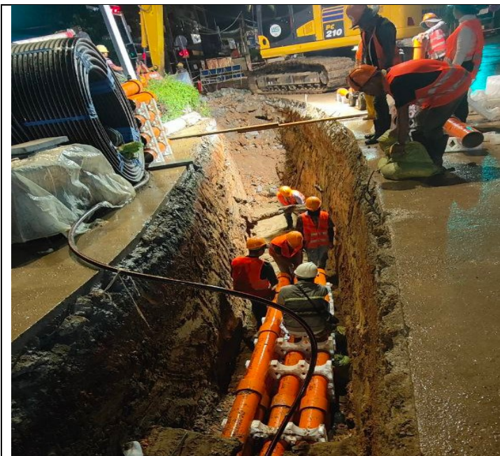
Photo: 19 Assembly PFP pipes and OFC pipe
