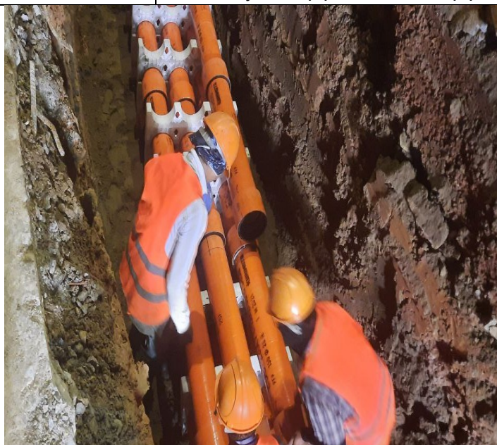
Photo: 24 Assembly PFP pipes and OFC pipe
