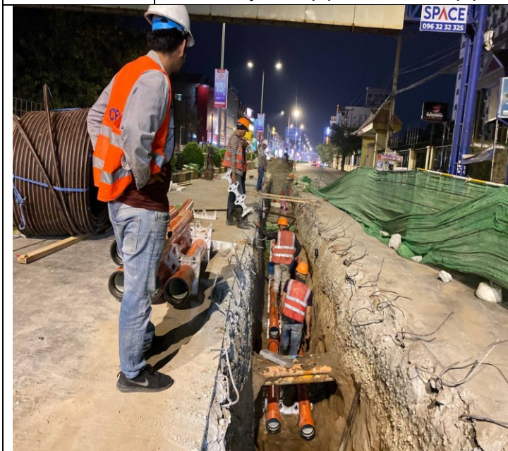
Photo: 11 Assembly PFP pipes and OFC pipe
