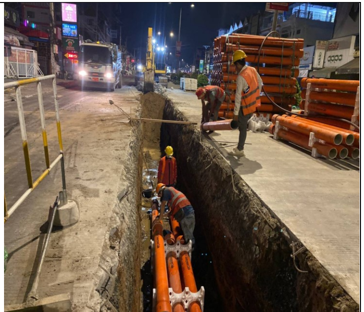
Photo: 14 Assembly PFP pipes and OFC pipe
