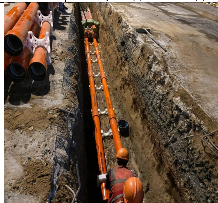
Photo: 17 Assembly PFP pipes and OFC pipe
