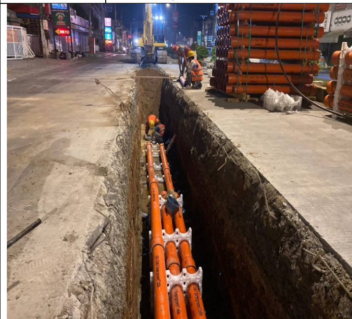
Photo: 15 Assembly PFP pipes and OFC pipe
