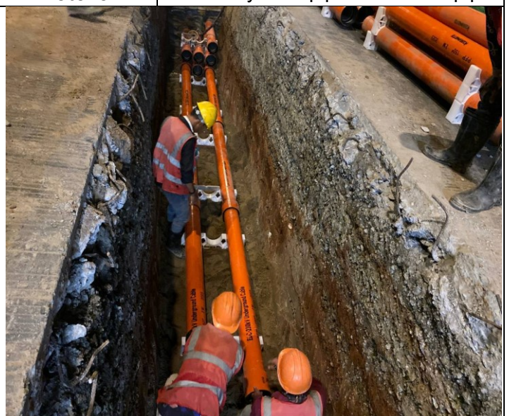
Photo: 06 Assembly PFP pipes and OFC pipe
