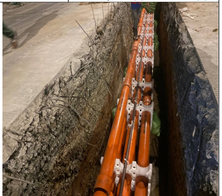
Photo: 12 Assembly PFP pipes and OFC pipe
