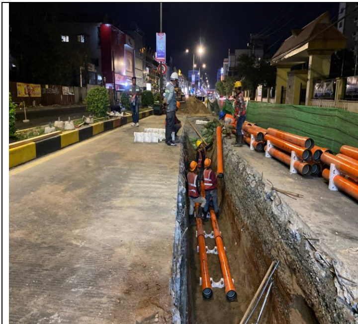
Photo: 07 Assembly PFP pipes and OFC pipe
