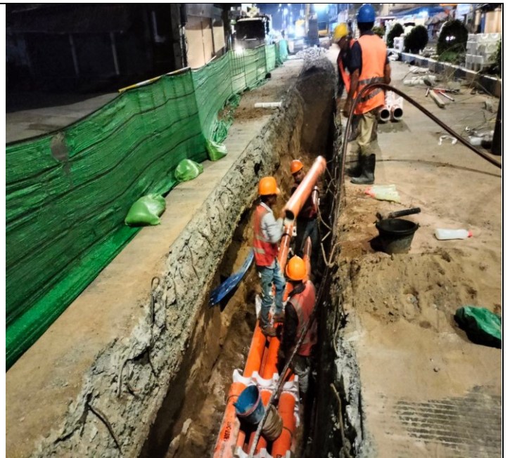
Photo: 08 Assembly PFP pipes and OFC pipe
