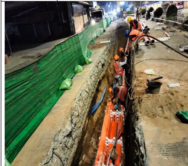
Photo: 09 Assembly PFP pipes and OFC pipe
