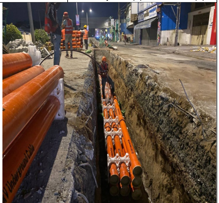
Photo: 18 Assembly PFP pipes and OFC pipe
