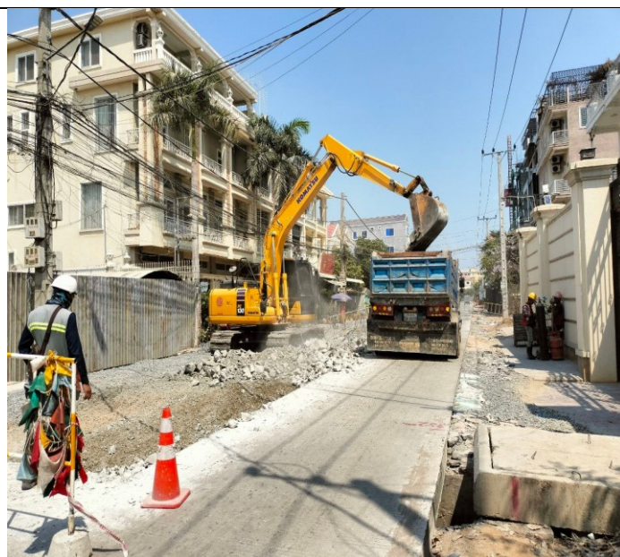
Photo: 20 Soil excavation and concrete road
