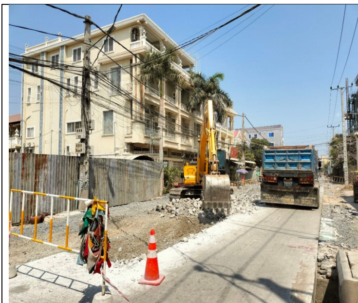
Photo: 19 Soil excavation and concrete road
