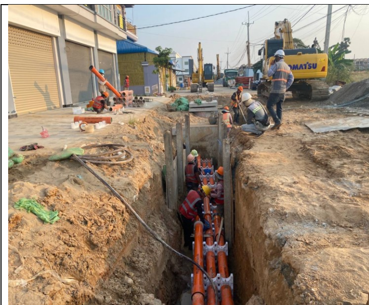
Photo: 19 | Assembly PFP pipes and OFC pipe
