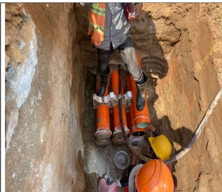
Photo: 13 Assembly PFP pipes and OFC pipe
