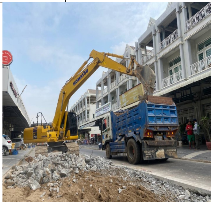
Photo: 12 Soil excavation and concrete road
